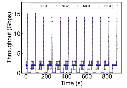
Figure 7: Traffic burst cycles of RNICs in a typical training container.
